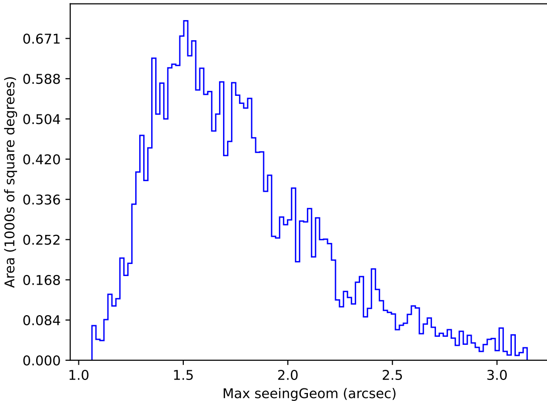
scp_reweight_v3.3_10yrs Yr 1 all bands: Max seeingGeom
