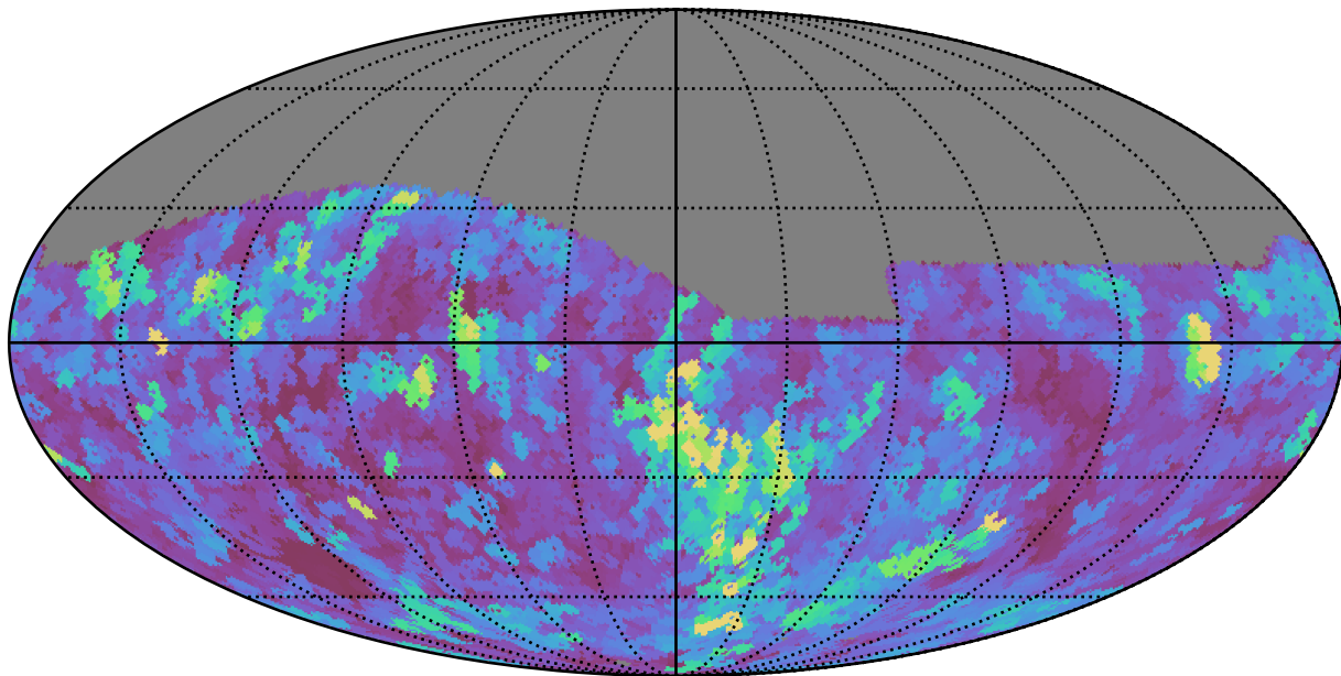
scp_reweight_v3.3_10yrs Yr 1 z band: Max seeingEff
