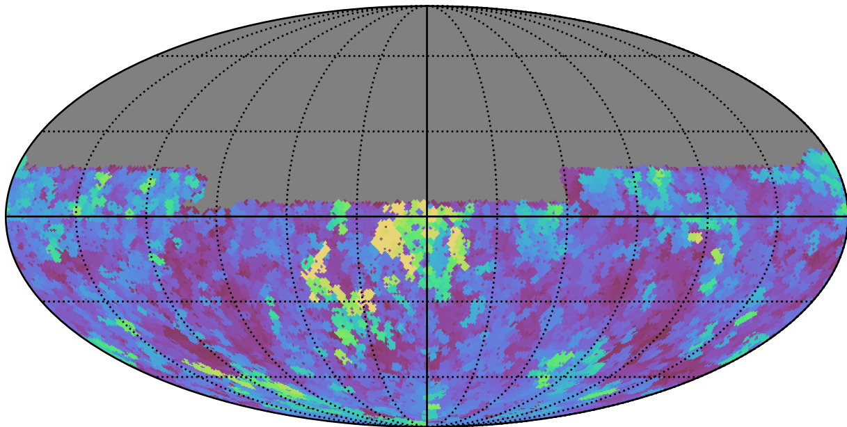
scp_reweight_v3.3_10yrs Yr 1 y band: Max seeingEff
