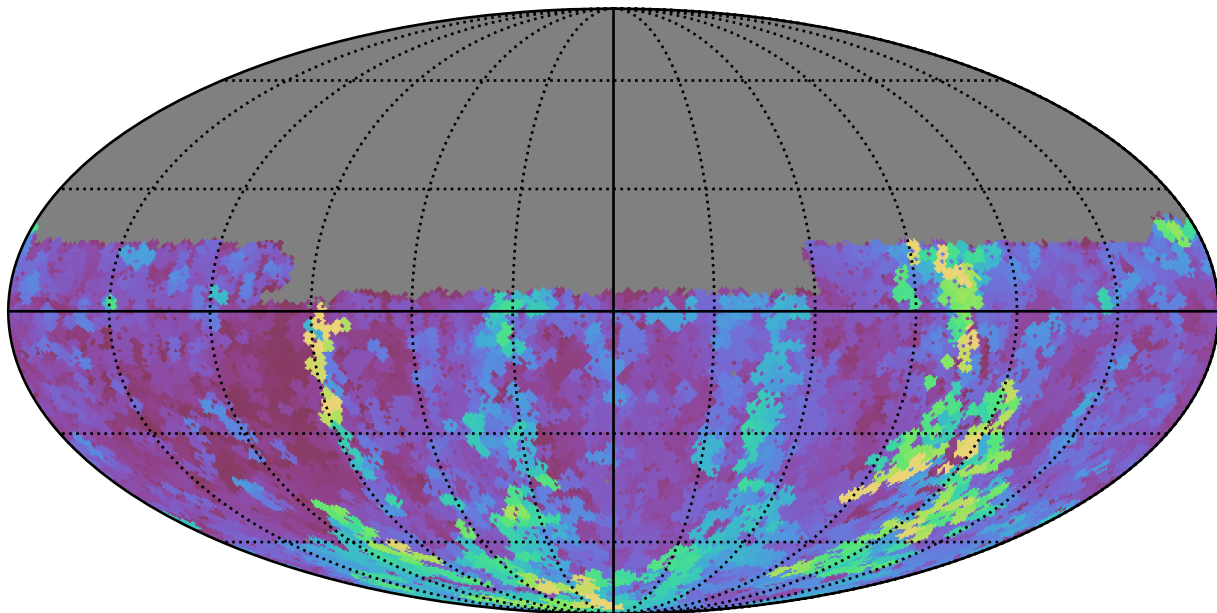
scp_reweight_v3.3_10yrs Yr 1 u band: Max seeingEff
