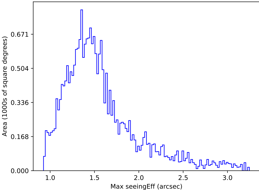
scp_reweight_v3.3_10yrs Yr 1 u band: Max seeingEff
