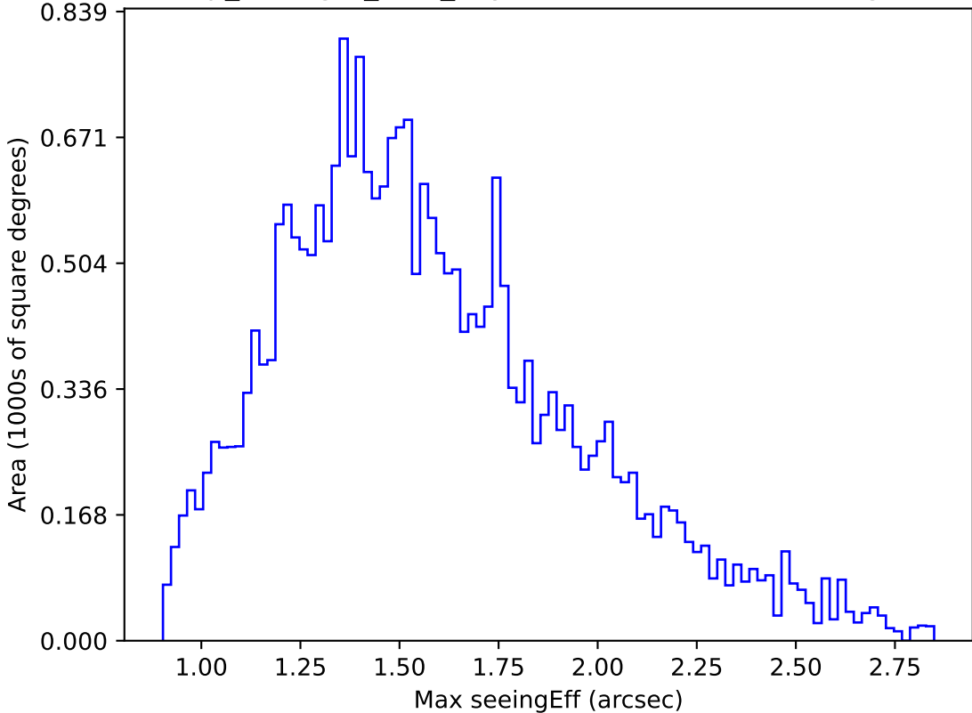
scp_reweight_v3.3_10yrs Yr 1 r band: Max seeingEff
