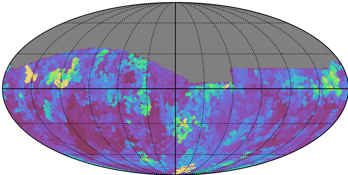
scp_reweight_v3.3_10yrs Yr 1 i band: Max seeingEff
