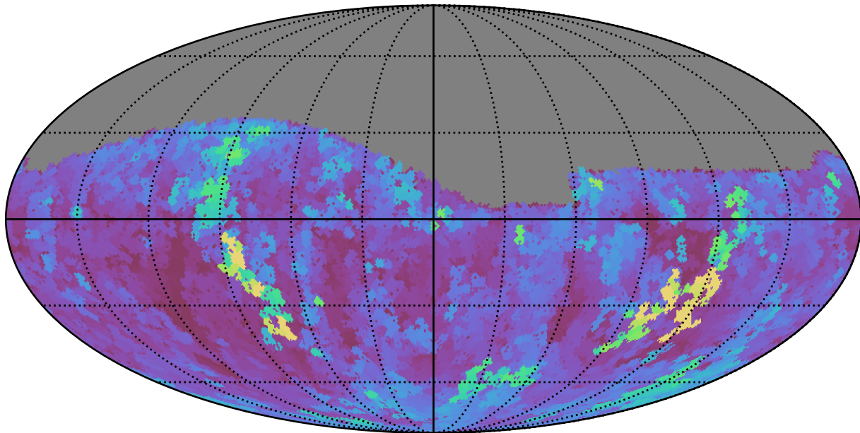
scp_reweight_v3.3_10yrs Yr 1 g band: Max seeingEff
