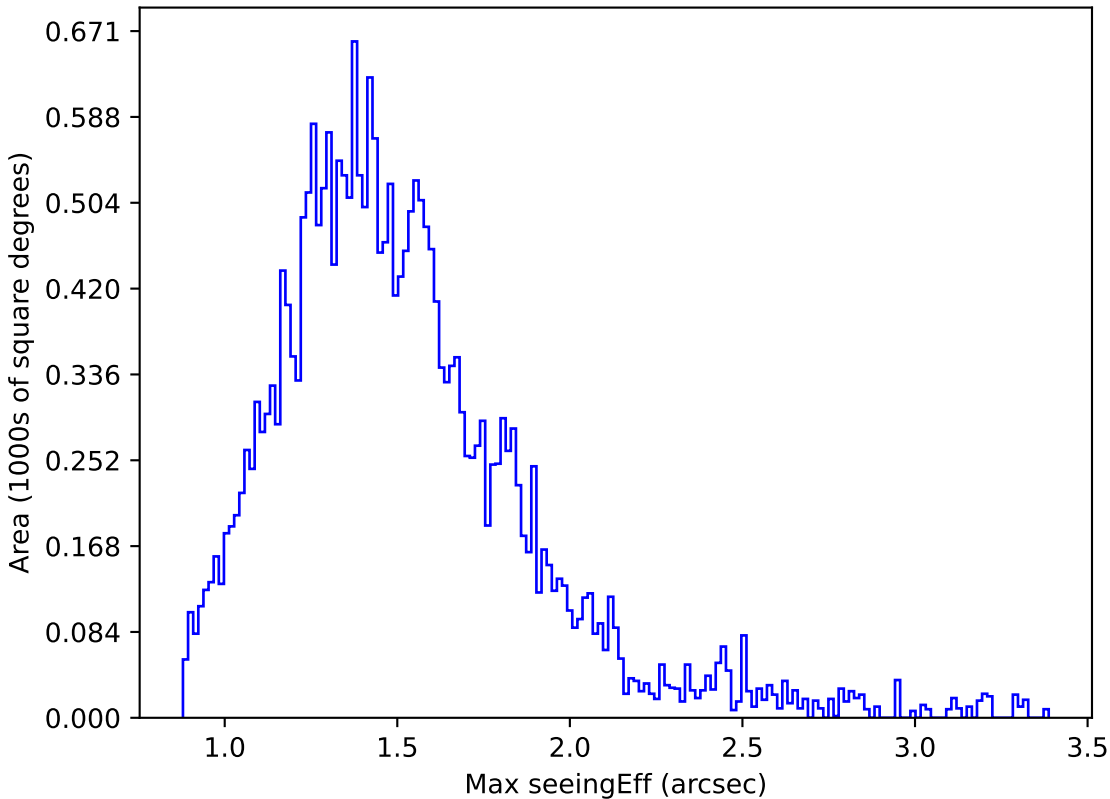
scp_reweight_v3.3_10yrs Yr 1 g band: Max seeingEff
