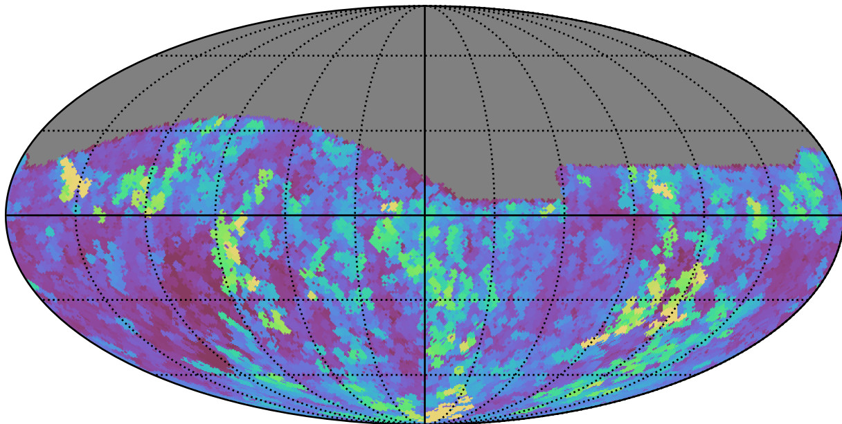
scp_reweight_v3.3_10yrs Yr 1 all bands: Max seeingEff
