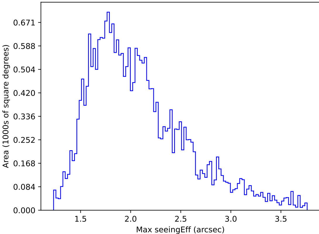
scp_reweight_v3.3_10yrs Yr 1 all bands: Max seeingEff
