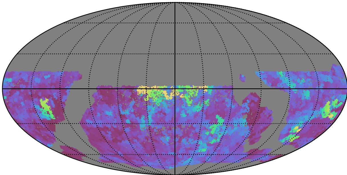
scp_reweight_v3.3_10yrs WFD y band: Max seeingEff
