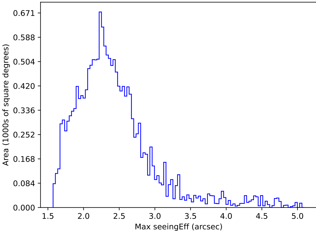
scp_reweight_v3.3_10yrs WFD y band: Max seeingEff
