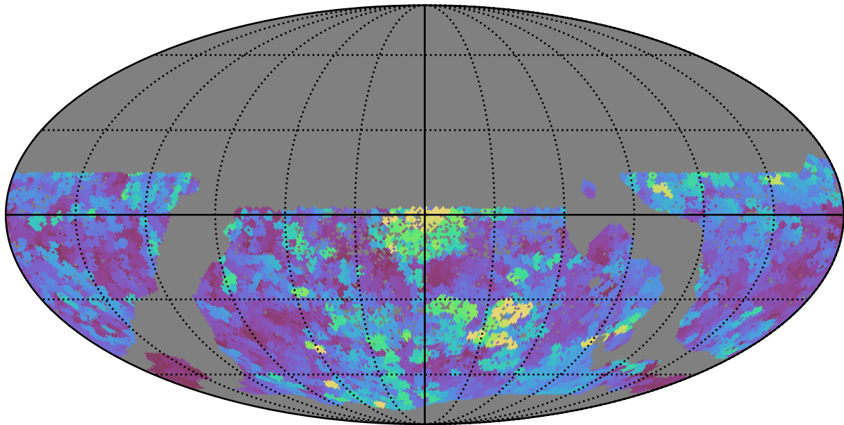
scp_reweight_v3.3_10yrs WFD u band: Max seeingEff
