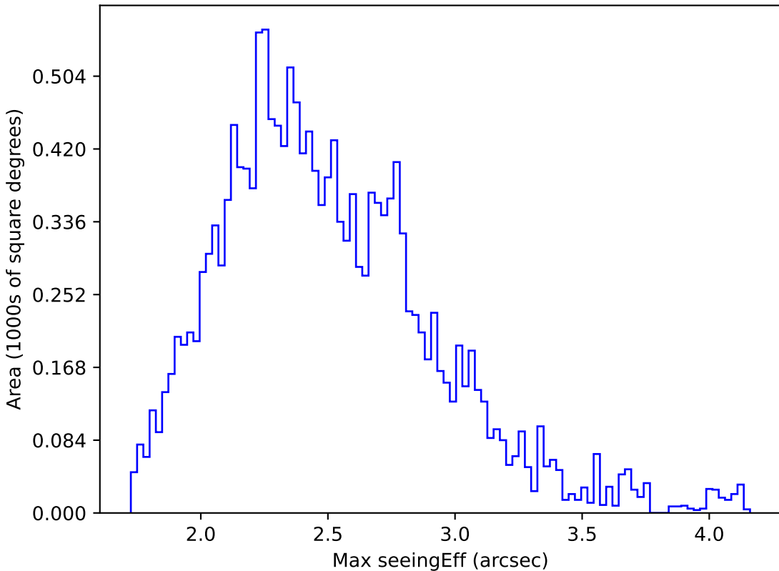
scp_reweight_v3.3_10yrs WFD u band: Max seeingEff
