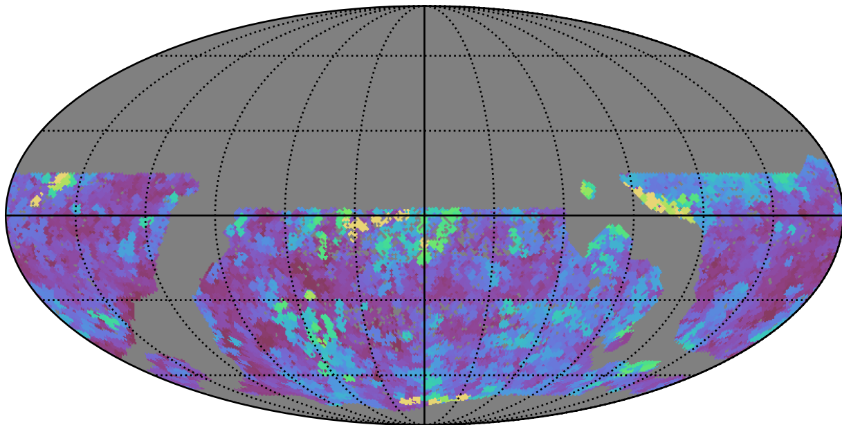
scp_reweight_v3.3_10yrs WFD r band: Max seeingEff
