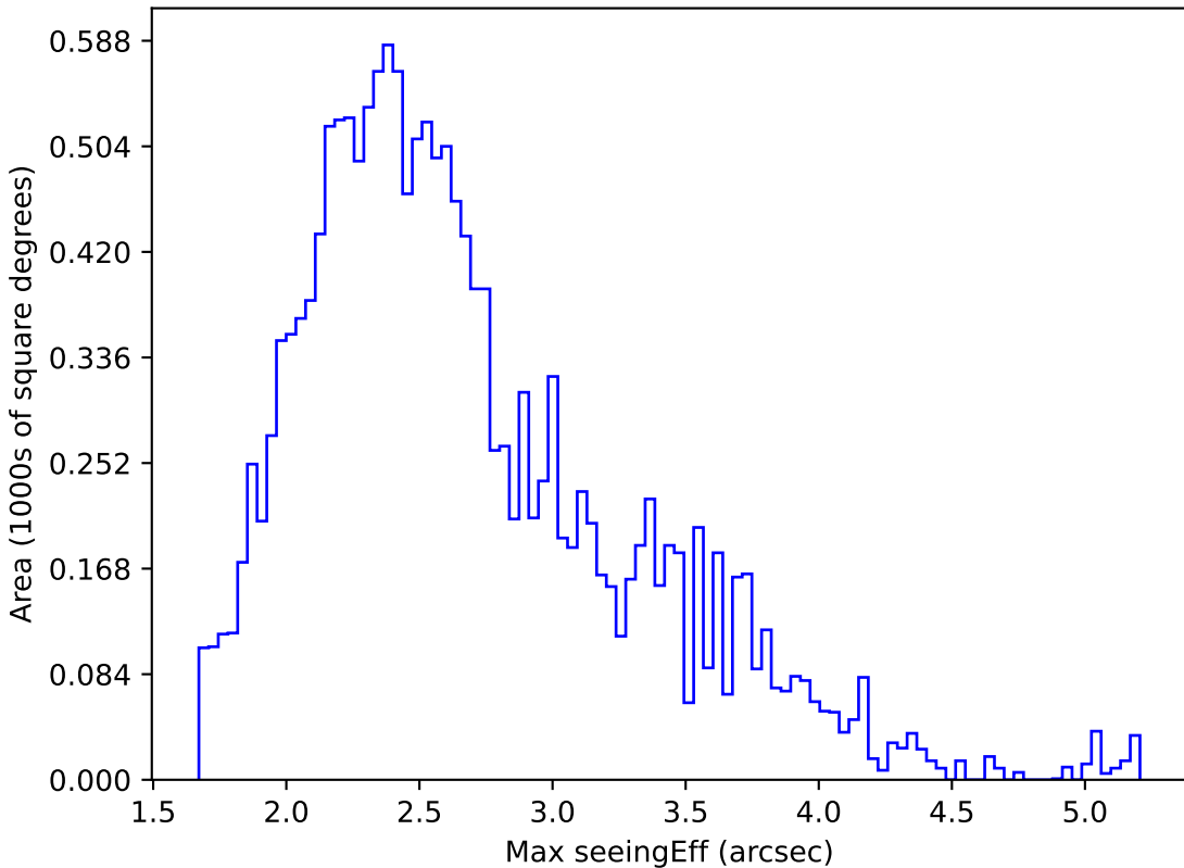
scp_reweight_v3.3_10yrs WFD i band: Max seeingEff
