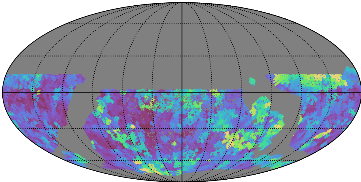
scp_reweight_v3.3_10yrs WFD g band: Max seeingEff
