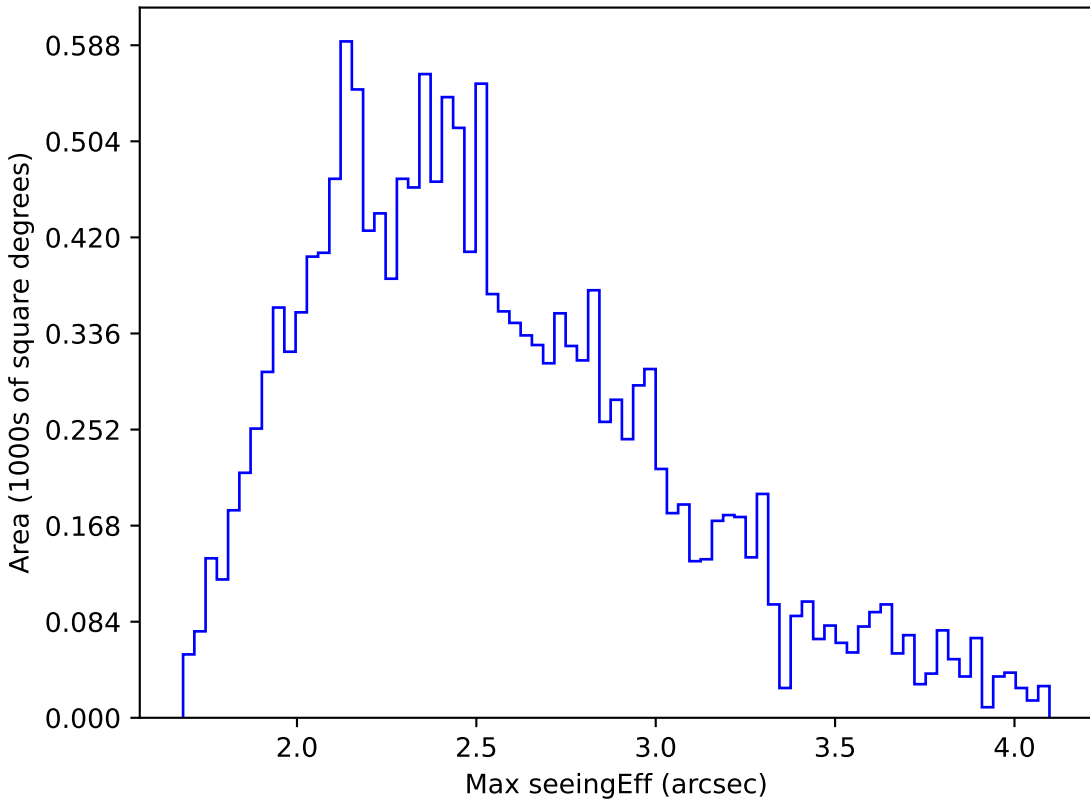
scp_reweight_v3.3_10yrs WFD g band: Max seeingEff
