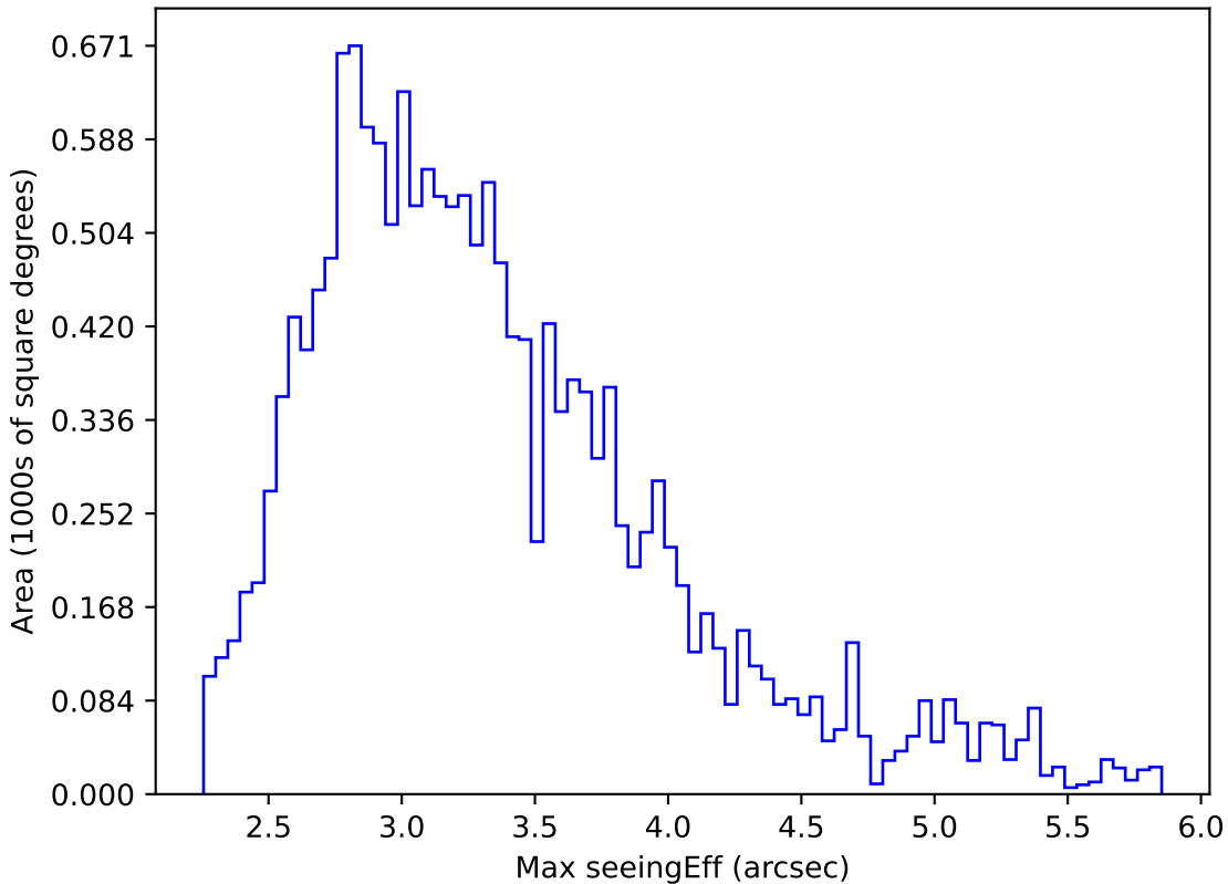
scp_reweight_v3.3_10yrs WFD all bands: Max seeingEff
