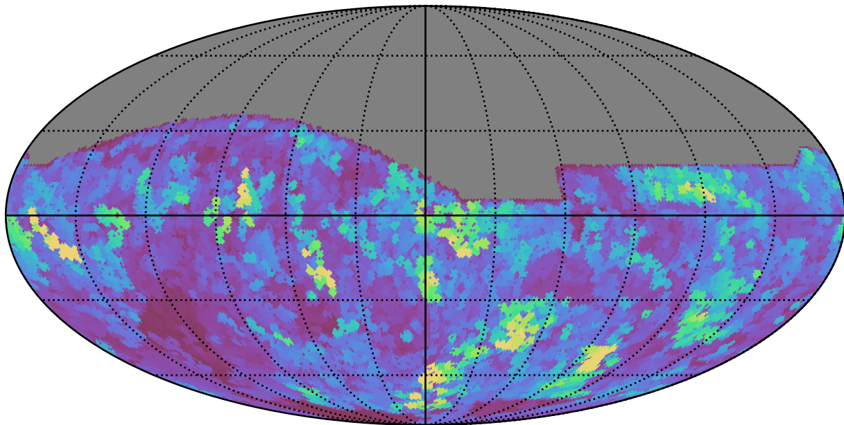
scp_reweight_v3.3_10yrs All sky z band: Max seeingEff
