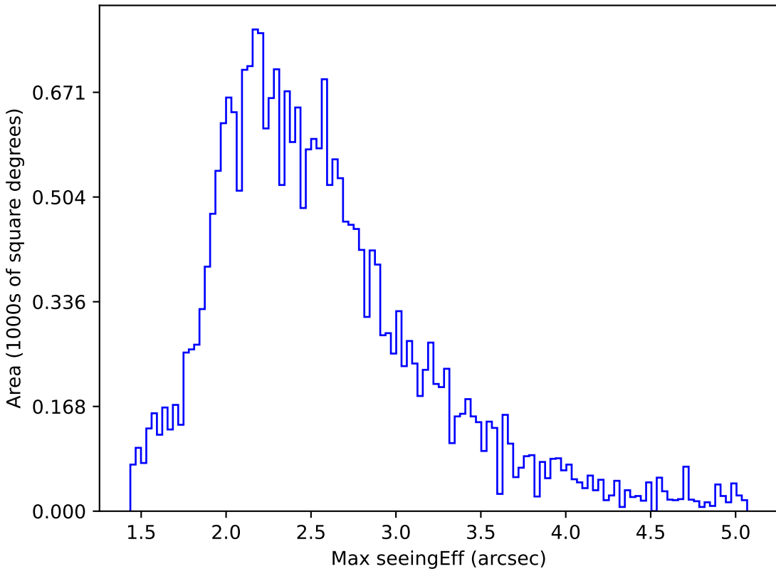
scp_reweight_v3.3_10yrs All sky z band: Max seeingEff
