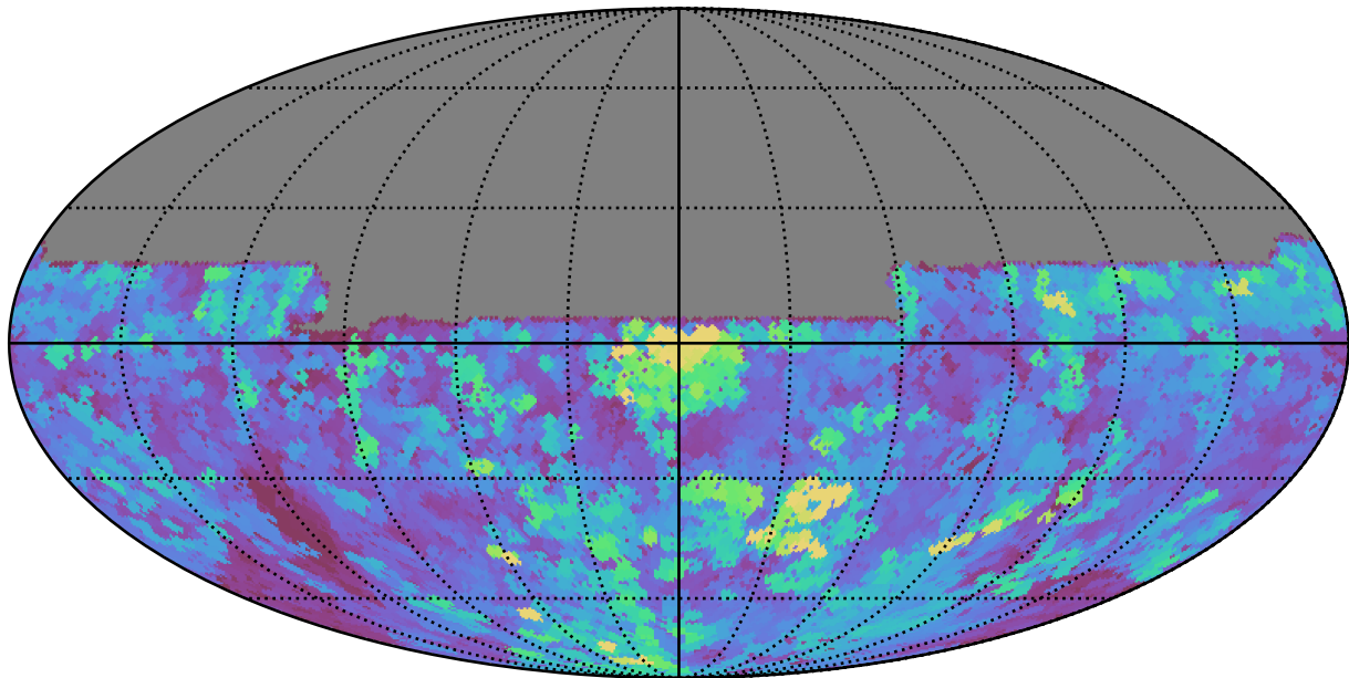
scp_reweight_v3.3_10yrs All sky u band: Max seeingEff
