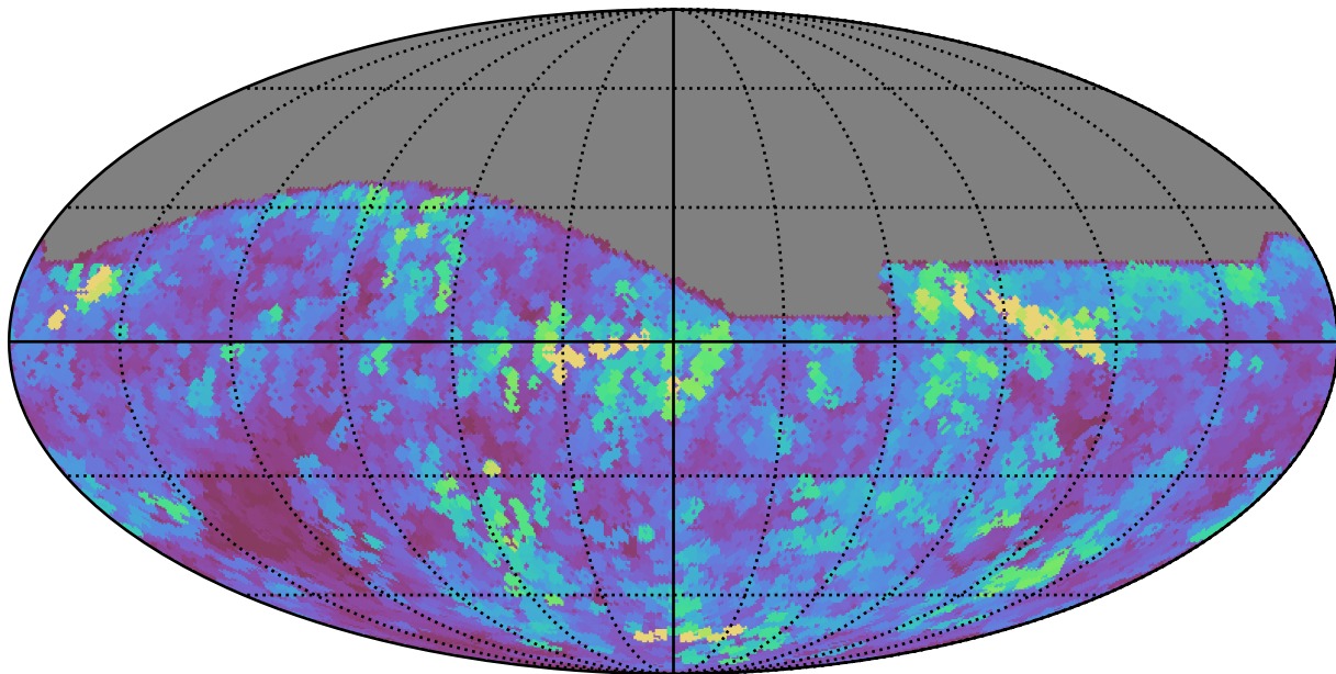
scp_reweight_v3.3_10yrs All sky r band: Max seeingEff
