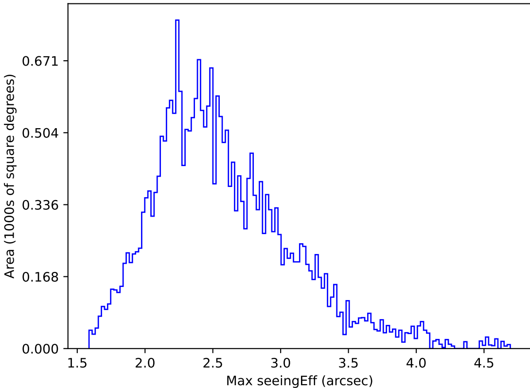
scp_reweight_v3.3_10yrs All sky r band: Max seeingEff
