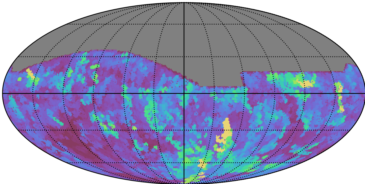
scp_reweight_v3.3_10yrs All sky i band: Max seeingEff
