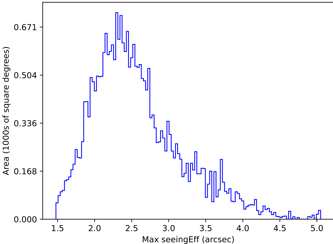
scp_reweight_v3.3_10yrs All sky i band: Max seeingEff
