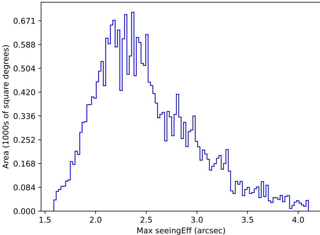
scp_reweight_v3.3_10yrs All sky g band: Max seeingEff
