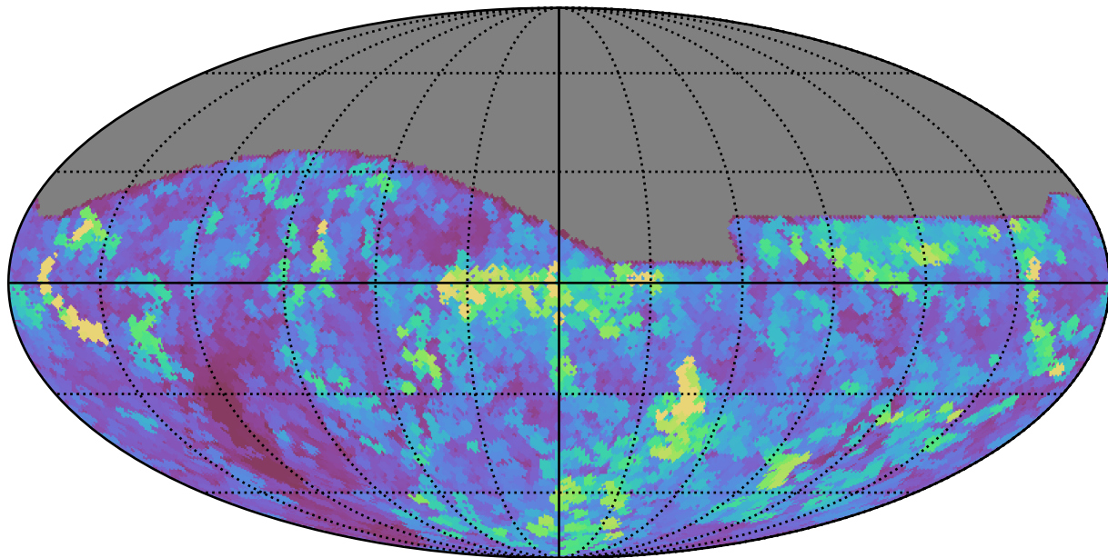
scp_reweight_v3.3_10yrs All sky all bands: Max seeingEff
