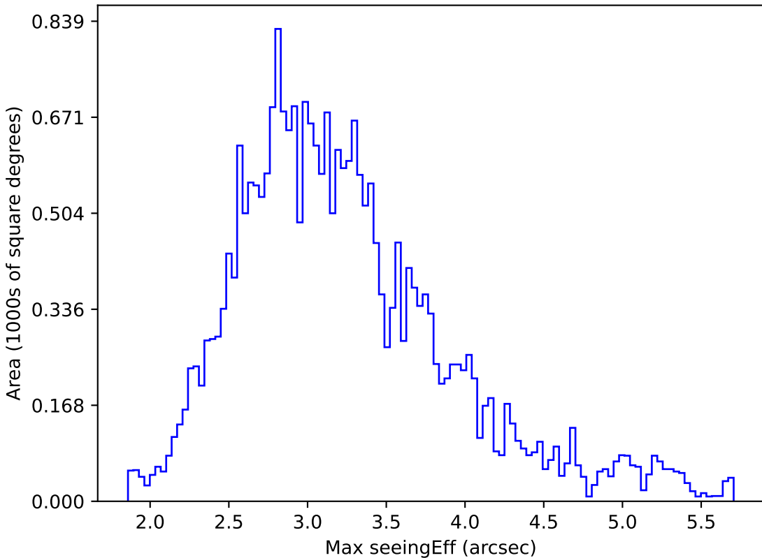
scp_reweight_v3.3_10yrs All sky all bands: Max seeingEff
