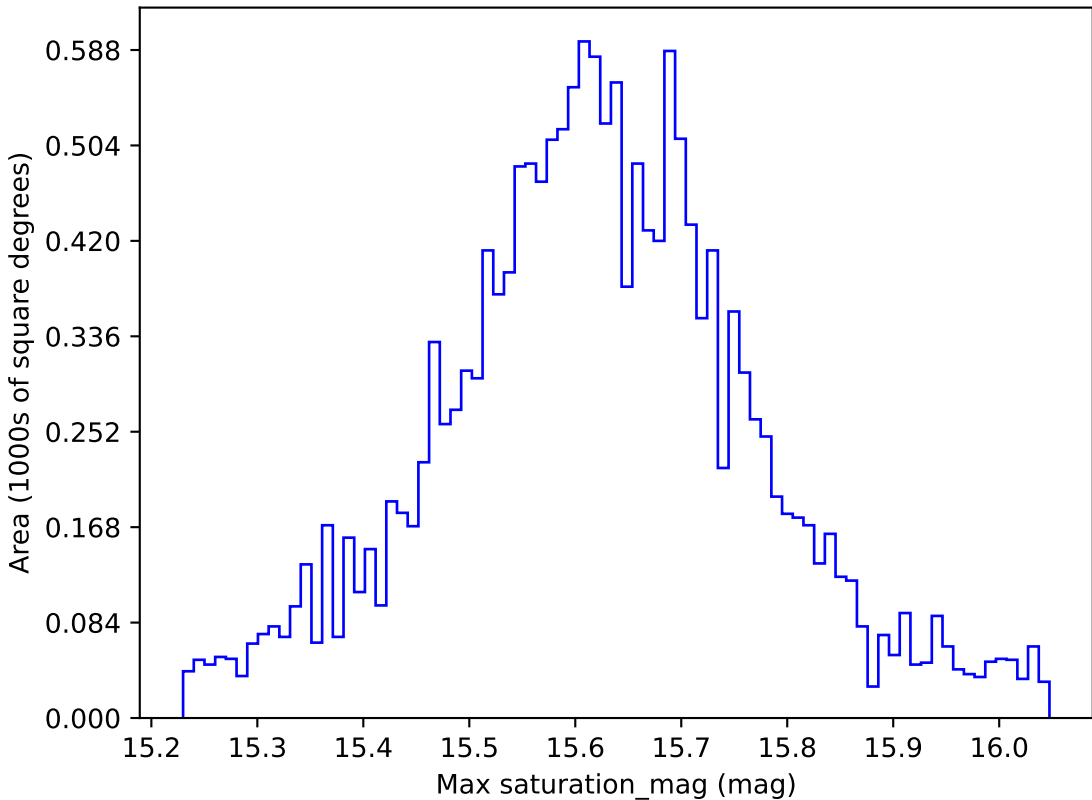
scp_reweight_v3.3_10yrs WFD i band: Max saturation_mag
