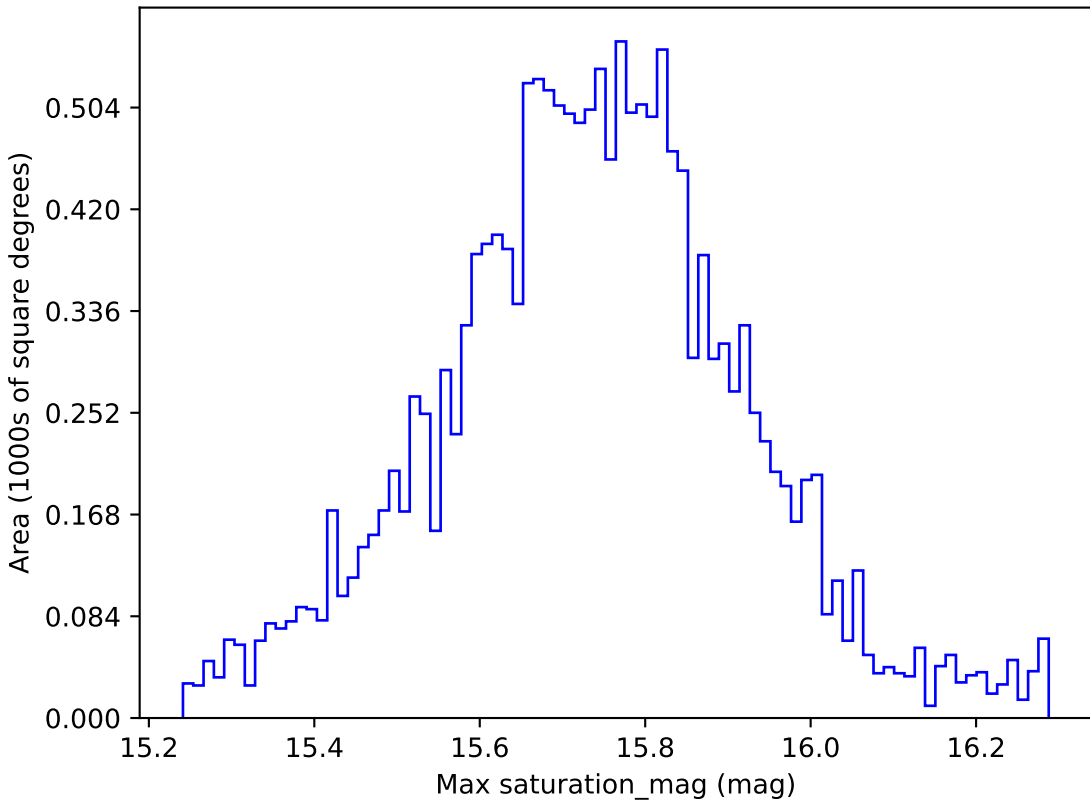
scp_reweight_v3.3_10yrs WFD g band: Max saturation_mag
