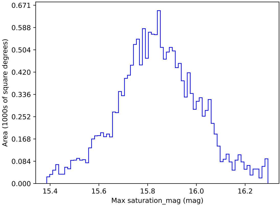
scp_reweight_v3.3_10yrs WFD all bands: Max saturation_mag
