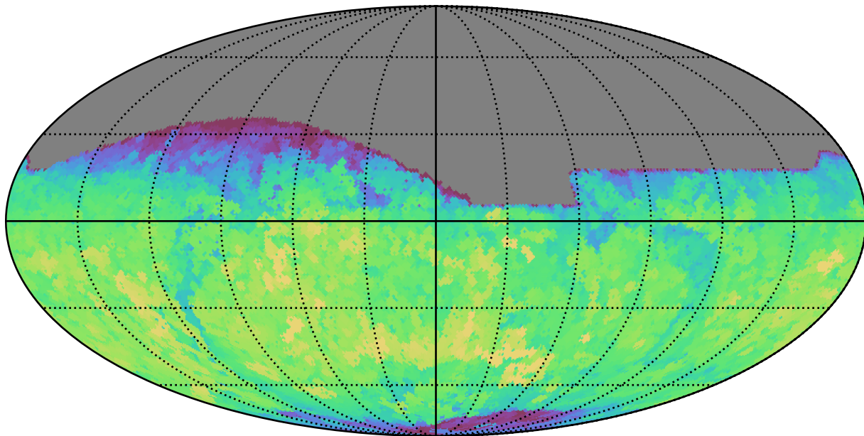
scp_reweight_v3.3_10yrs All sky z band: Max saturation_mag
