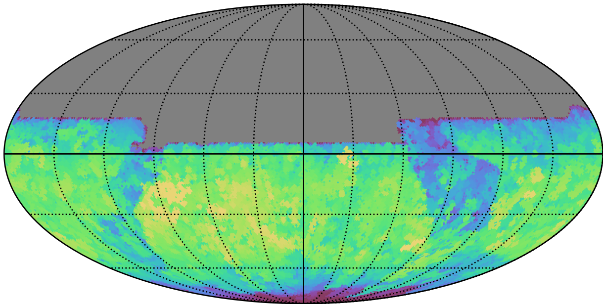
scp_reweight_v3.3_10yrs All sky y band: Max saturation_mag
