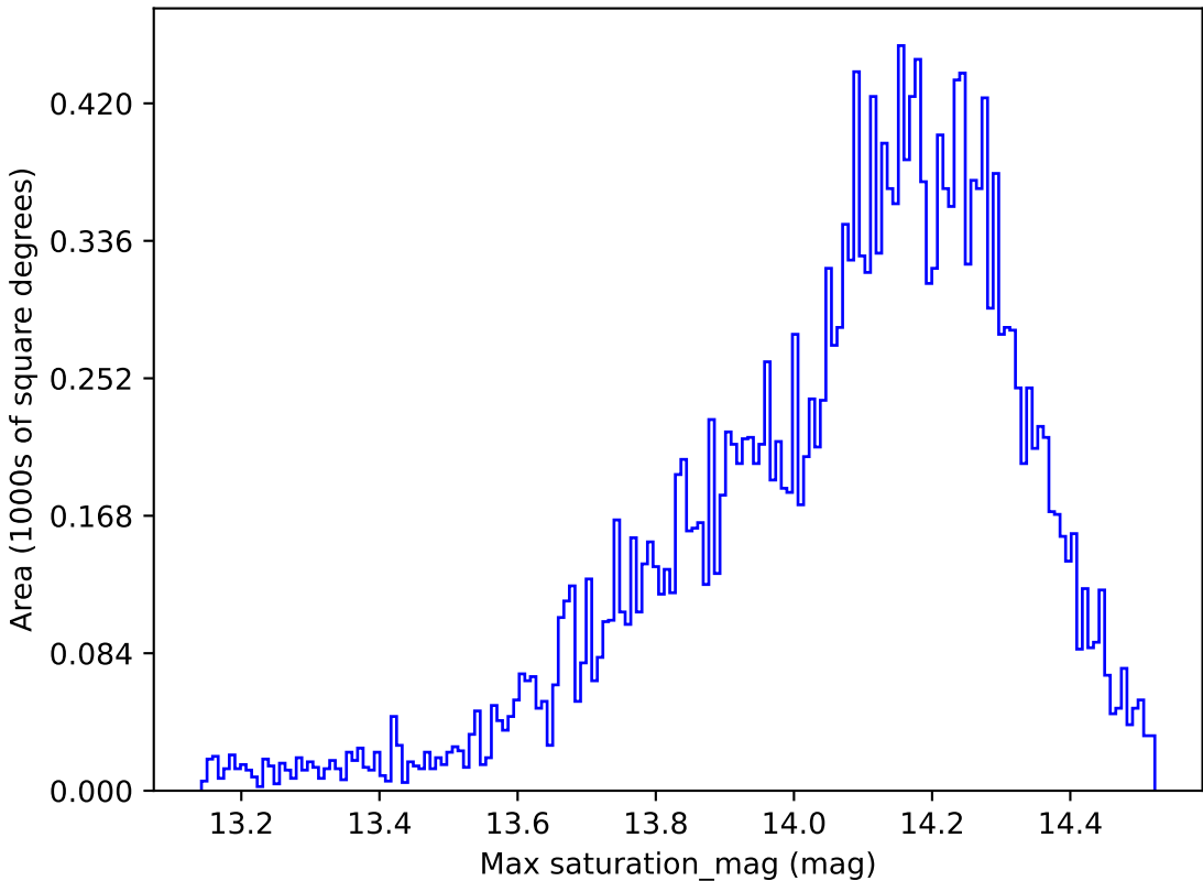
scp_reweight_v3.3_10yrs All sky y band: Max saturation_mag
