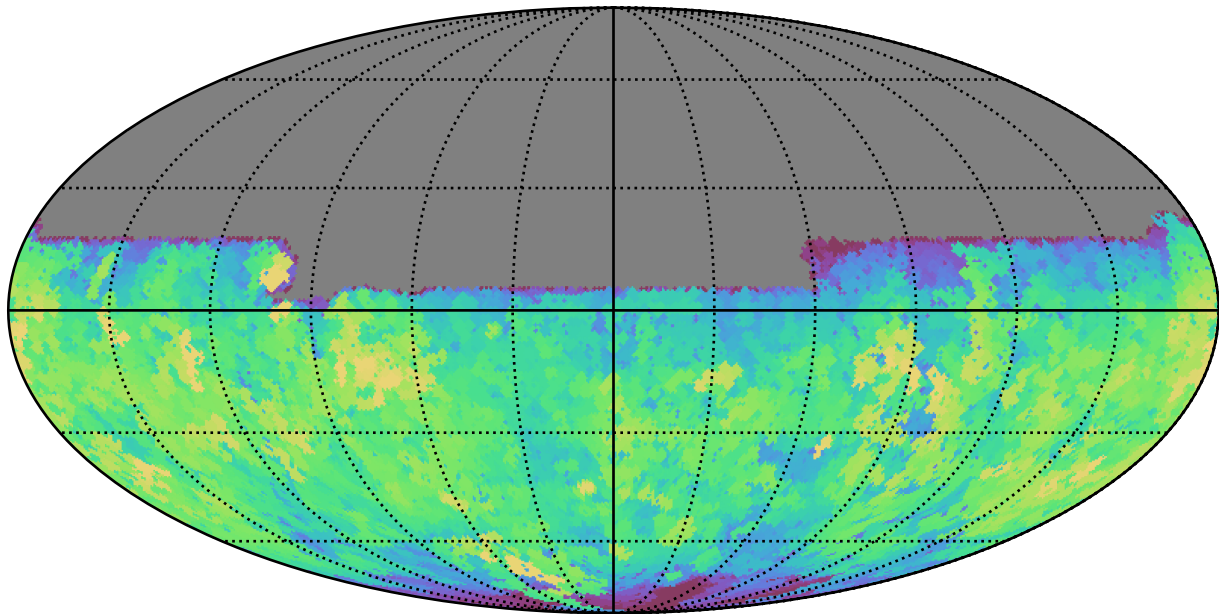
scp_reweight_v3.3_10yrs All sky u band: Max saturation_mag
