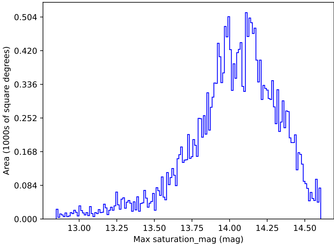
scp_reweight_v3.3_10yrs All sky u band: Max saturation_mag
