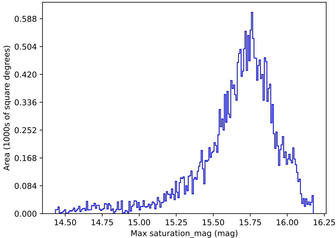
scp_reweight_v3.3_10yrs All sky r band: Max saturation_mag
