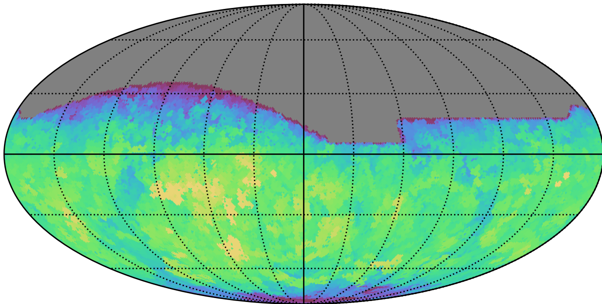
scp_reweight_v3.3_10yrs All sky i band: Max saturation_mag
