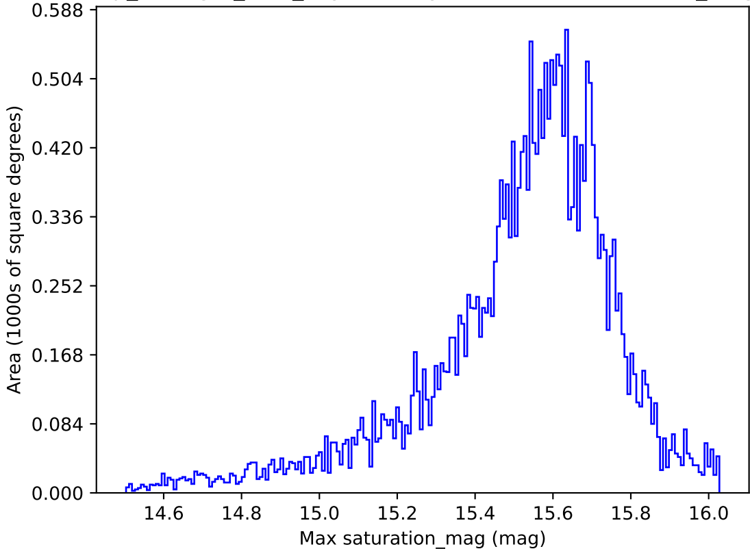
scp_reweight_v3.3_10yrs All sky i band: Max saturation_mag
