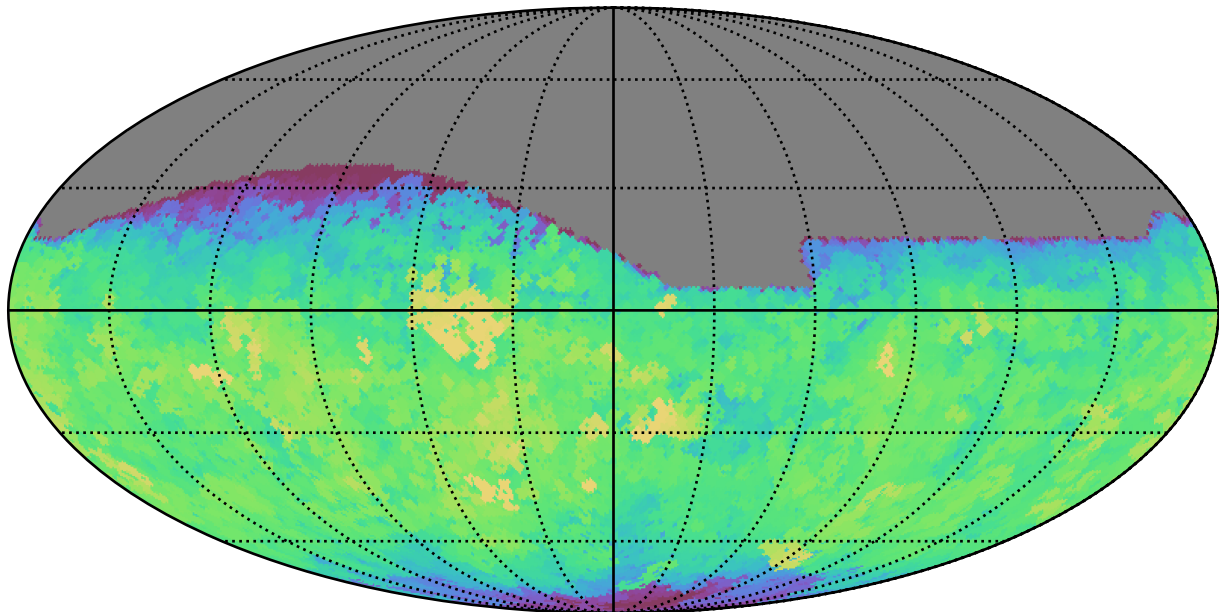
scp_reweight_v3.3_10yrs All sky g band: Max saturation_mag
