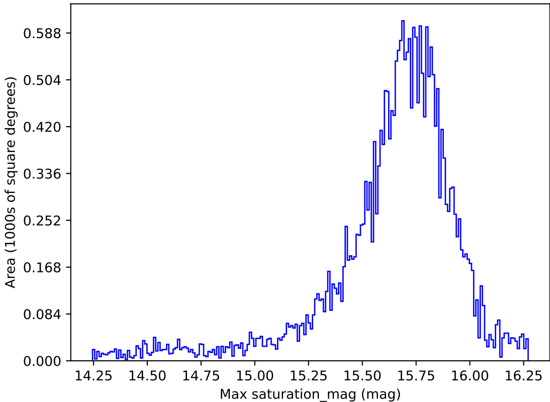
scp_reweight_v3.3_10yrs All sky g band: Max saturation_mag
