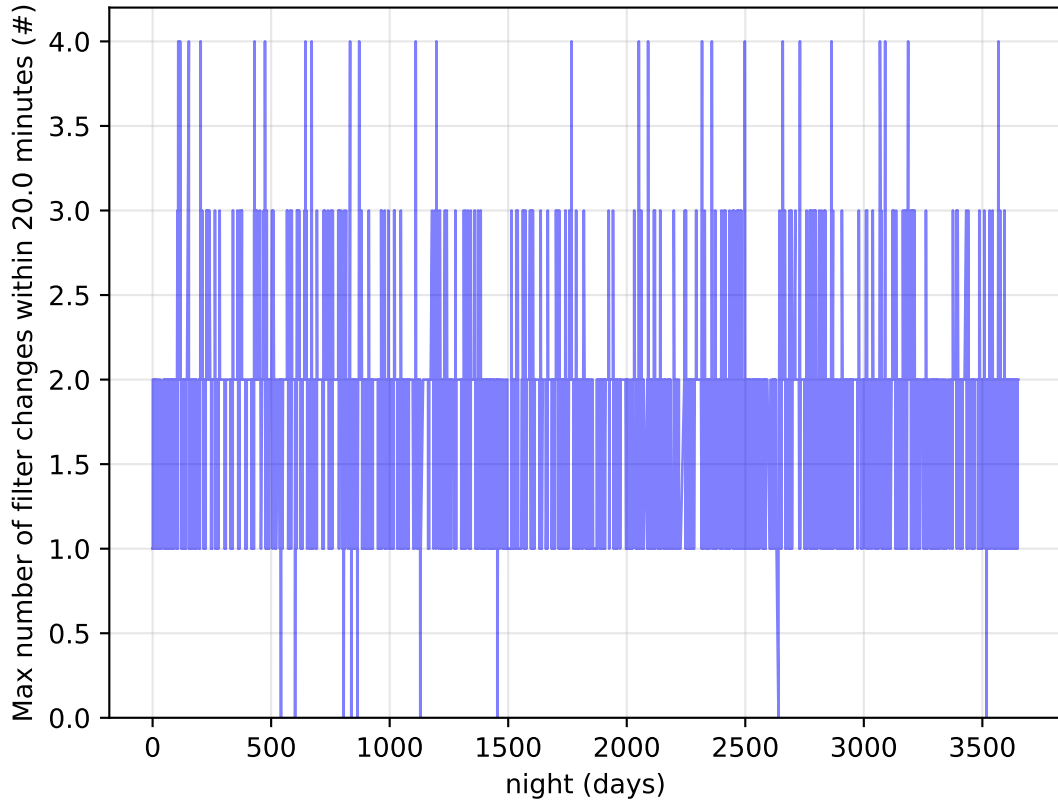
scp_reweight_v3.3_10yrs Per Night: Max number of filter changes within 20.0 minutes
