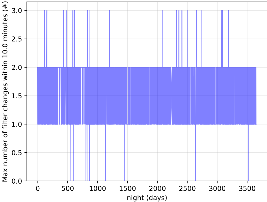
scp_reweight_v3.3_10yrs Per Night: Max number of filter changes within 10.0 minutes
