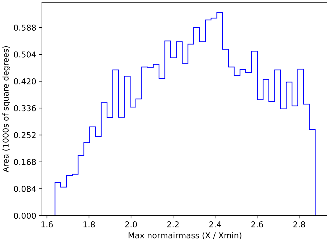
scp_reweight_v3.3_10yrs WFD z band: Max normairmass
