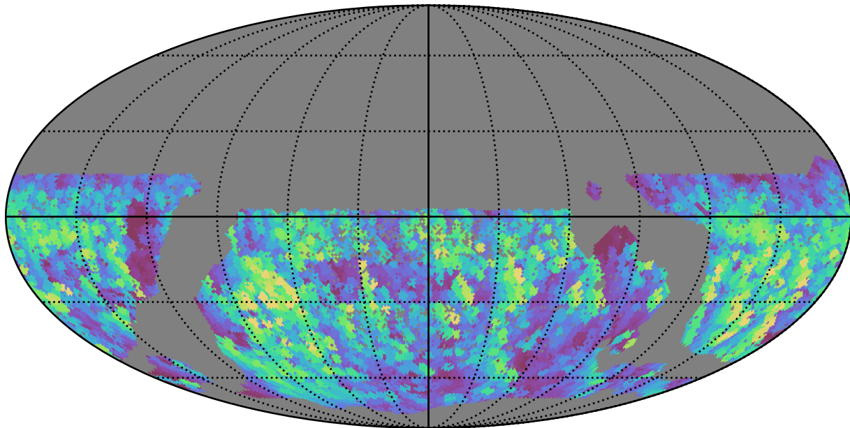
scp_reweight_v3.3_10yrs WFD y band: Max normairmass
