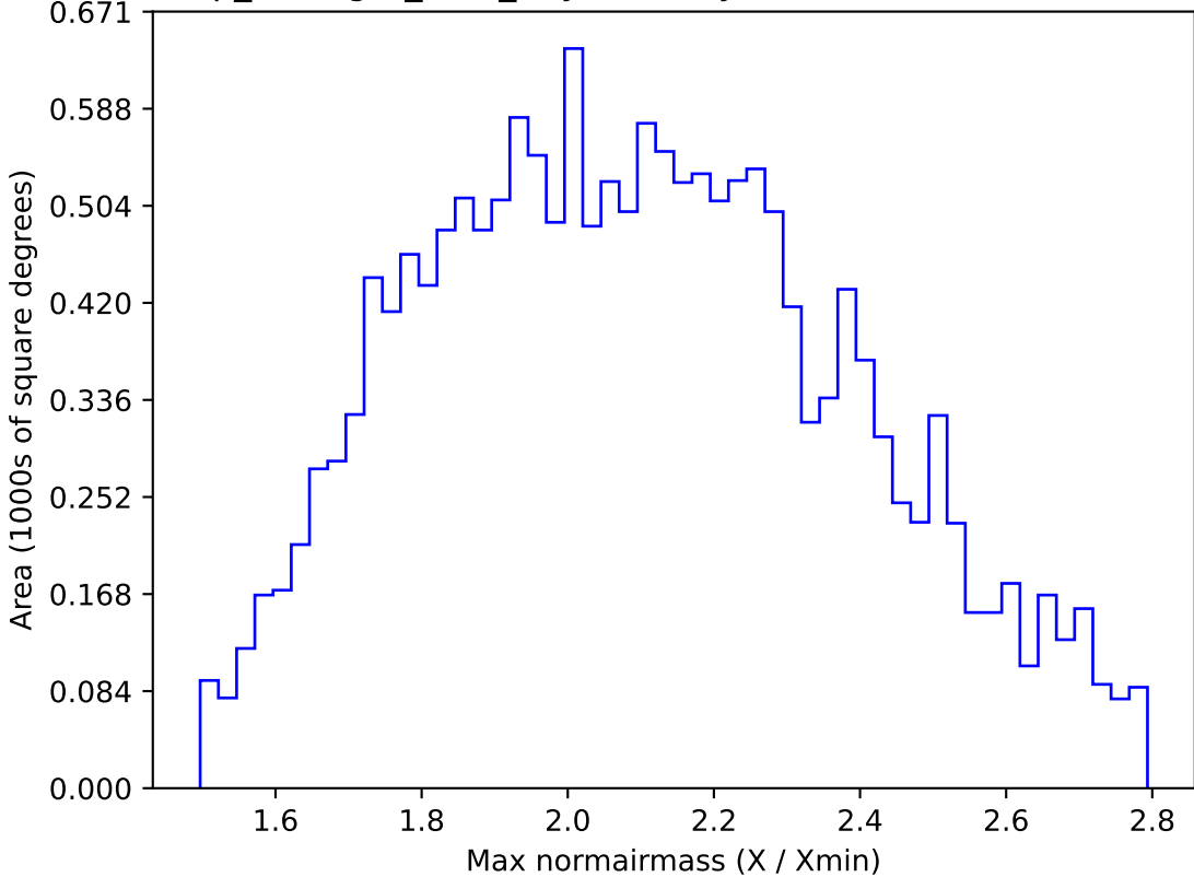
scp_reweight_v3.3_10yrs WFD y band: Max normairmass
