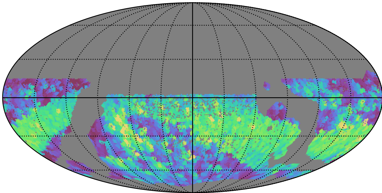
scp_reweight_v3.3_10yrs WFD r band: Max normairmass
