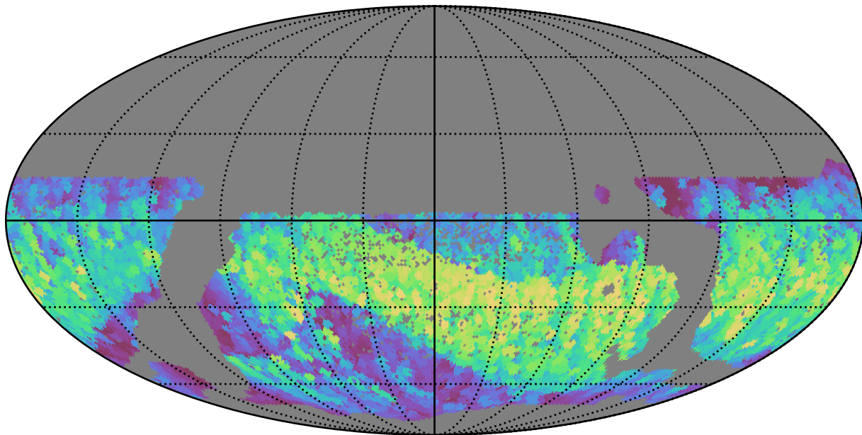
scp_reweight_v3.3_10yrs WFD i band: Max normairmass
